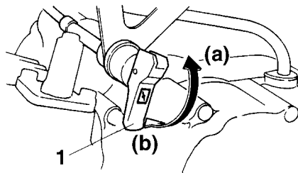
1. Commande de starter " |v| "
