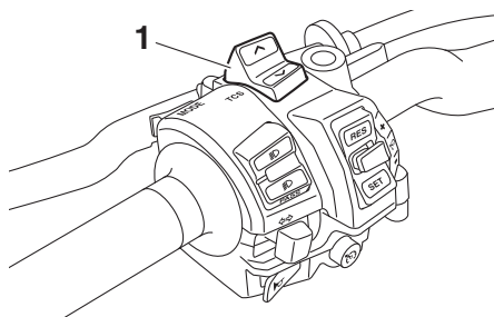
1. TCS-schakelaar “^/▼”
